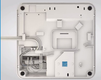
Effective Cable Management with Various Exits
